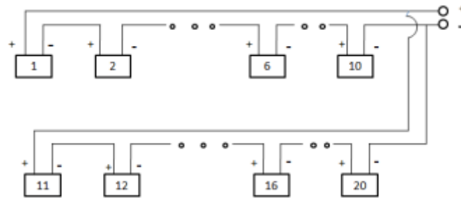
Figure 2: Connection Of Batteries
