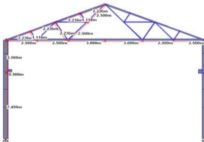
Figure No.4 Internal main frame with crane brackets
