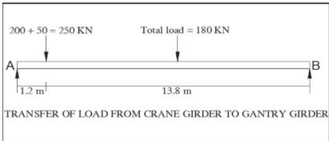
Figure No.1 maximum vertical static wheel load = 160 KN Taking the impact factor for an electrically operated traveling crane as per IS 875 as 25% Wheel load with impact factor = 200 KN
