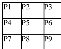
Fig. 3 3X3 neighborhood
