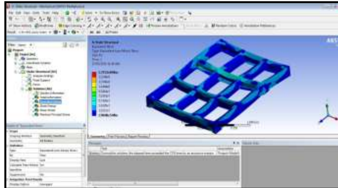
Fig.4.5 Normal Stress
