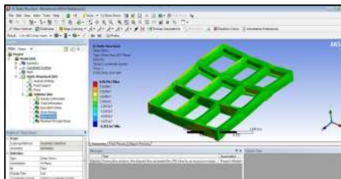
Fig.4.4 Shear Stress produced in Chassis
