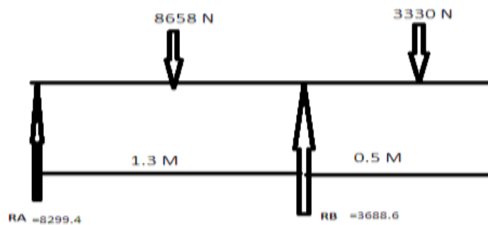
Fig.3.2 Load Diagram of Chassis
