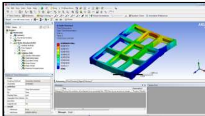
Fig.4.3 Total Deflection of Chassis
