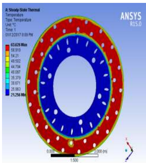
Fig -1 Temperature for profile i stainless steel
