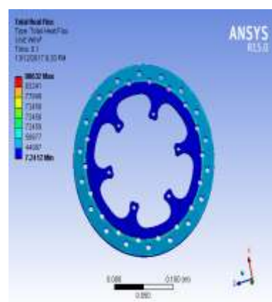
Fig -6 Total heat flux for profile ii stainless steel.
