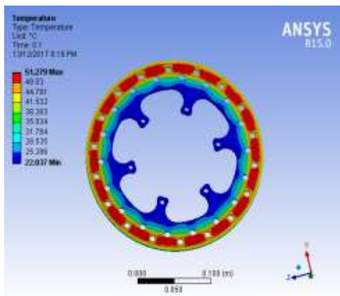
Fig -5 Temperature distribution for profile ii stainless steel.
