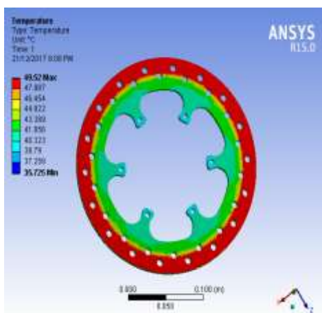
Fig -7 Temperature distribution for profile ii cast iron.
