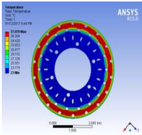
Fig -3 Temperature for profile i cast iron.
