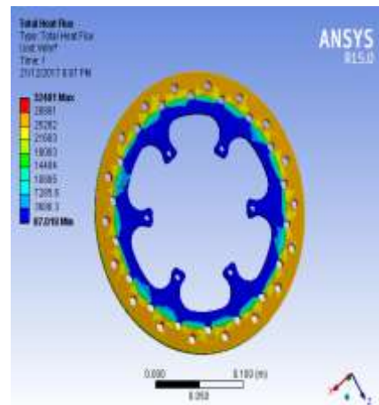
Fig - 8 Total heat flux for profile ii cast iron.
