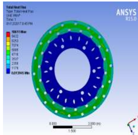
Fig -4 Total heat flux for profile i cast iron..
