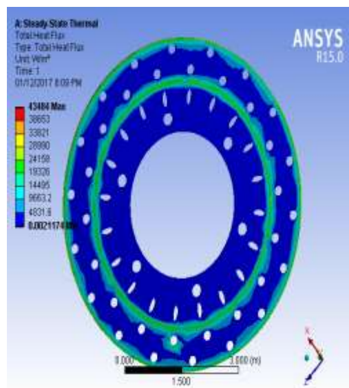
Fig -2 Total heat flux for profile i stainless steel.
