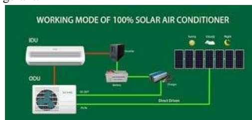
Fig. 2. Working Mode of 100% Solar Air Conditioner
