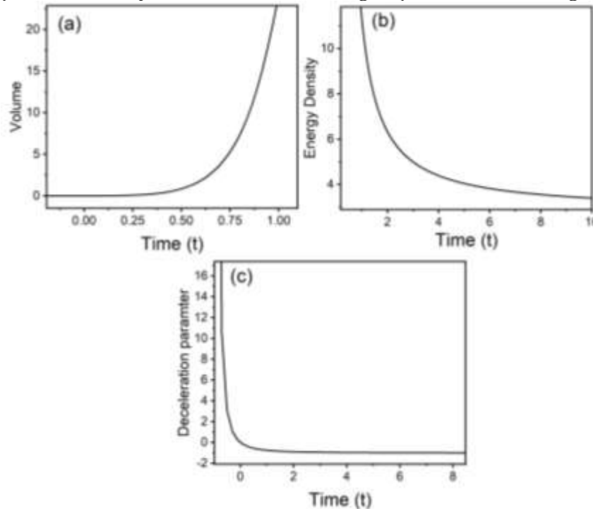
Fig -1 Plots of time versus (a) Spatial volume (b) Energy density (c) Deceleration parameter for the values r = 1, l = 1, m = 2 .
