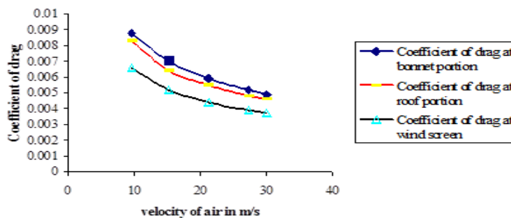
Figure 8, Variation of Co-efficient of Drag Force with Velocity of Air for Tata Indica Car
