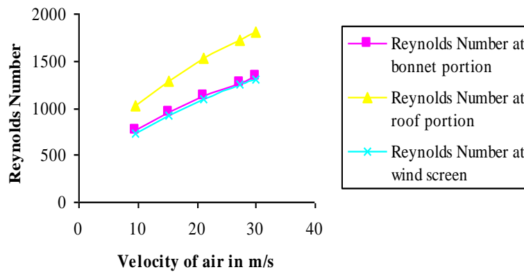
Figure 9, Variation of Reynolds Number with Velocity of Air for Tata Indica
