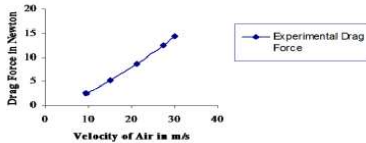
Figure 7, Relation between Experimental Drag force and Velocity of Air
