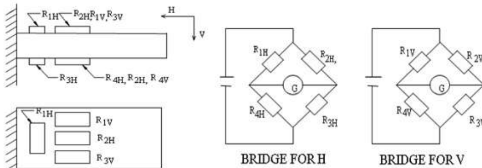
Figure 3, Configuration and Circuit Diagrams for Strain Gauge Mounting and Usage
