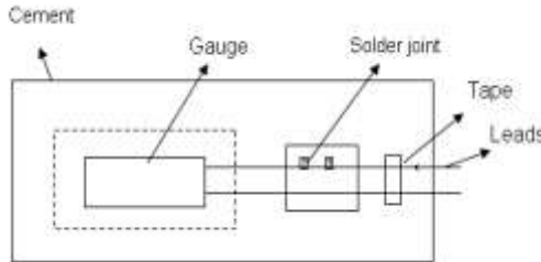
Figure2, Strain Gauge with Leads Connection
