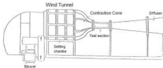
Figure 4, Wind Tunnel
