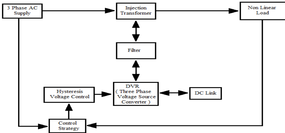
Fig -1 Schematic diagram of DVR
