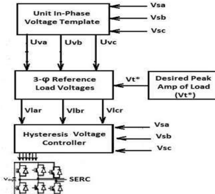
Fig -2 Control Scheme of DVR
