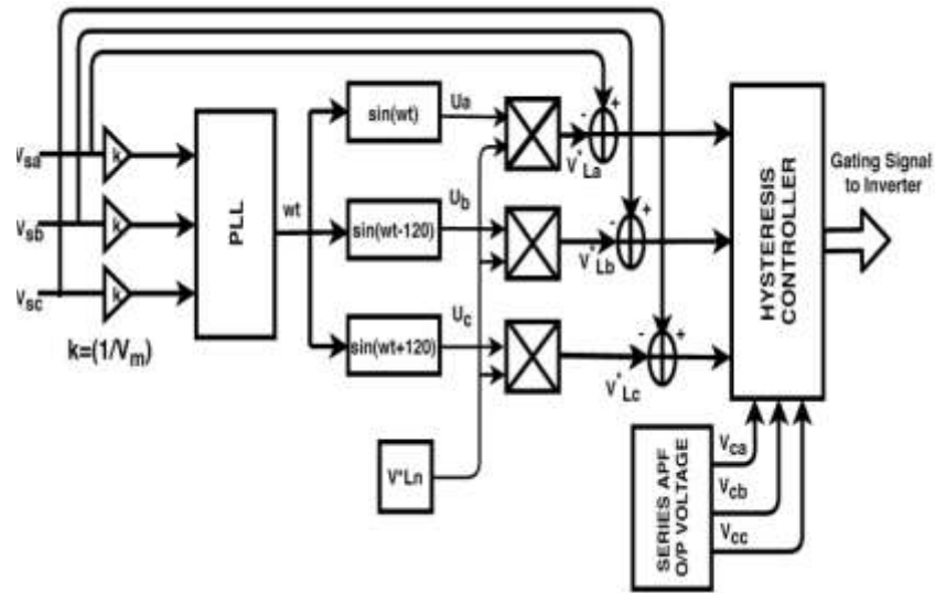
Fig -3 Control Block Diagram of DVR Using UVTG
