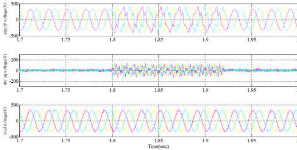
Fig -7 Simulation results of DVR under unbalanced voltage supply
