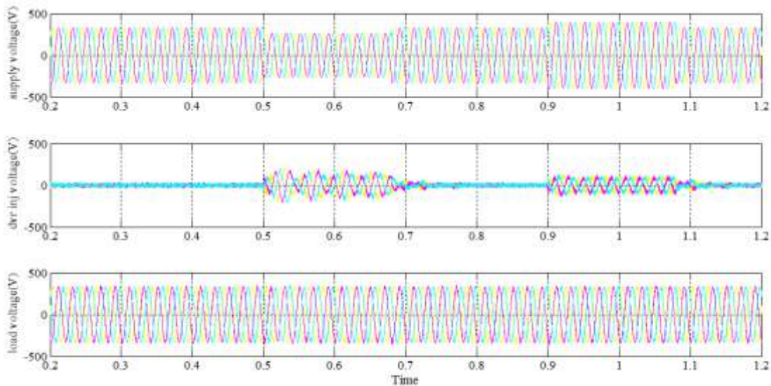
Fig -6 Simulation results of DVR under voltage sag (0.5-0.7) sec and swell (0.9-1.1) sec
