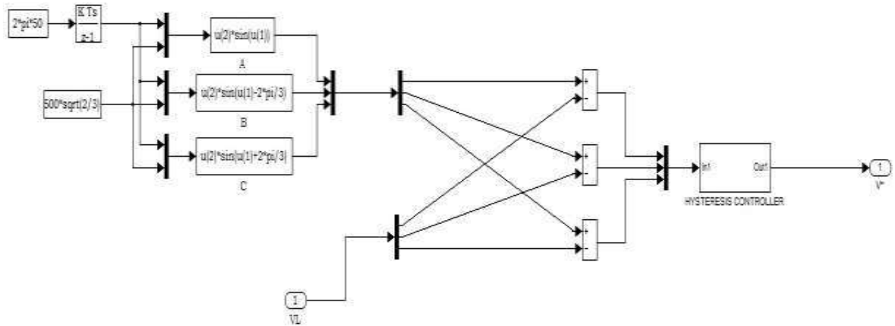
Fig -5 MATLAB Model of DVR Controller
