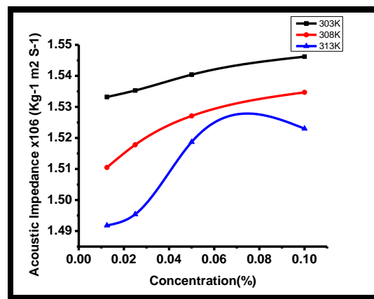
Fig.10:-Variation of Acoustic Impedance with concentration and temperature
