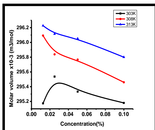
Fig.13:-Variation of Molar volume with concentration and temperature
