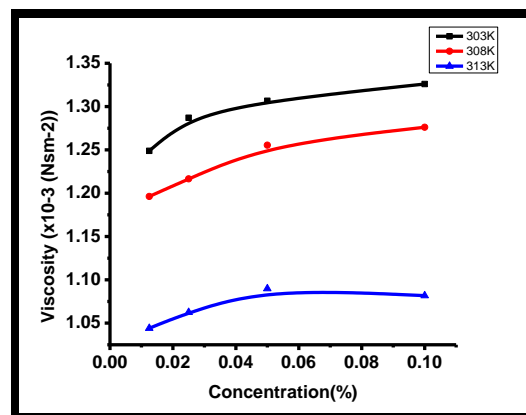
Fig.4:-Variation of Viscosity with concentration and temperature
