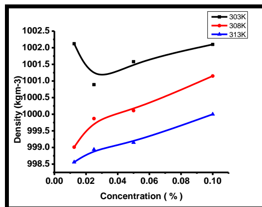
Fig.2:-Variation of Density with concentration and temperature.
