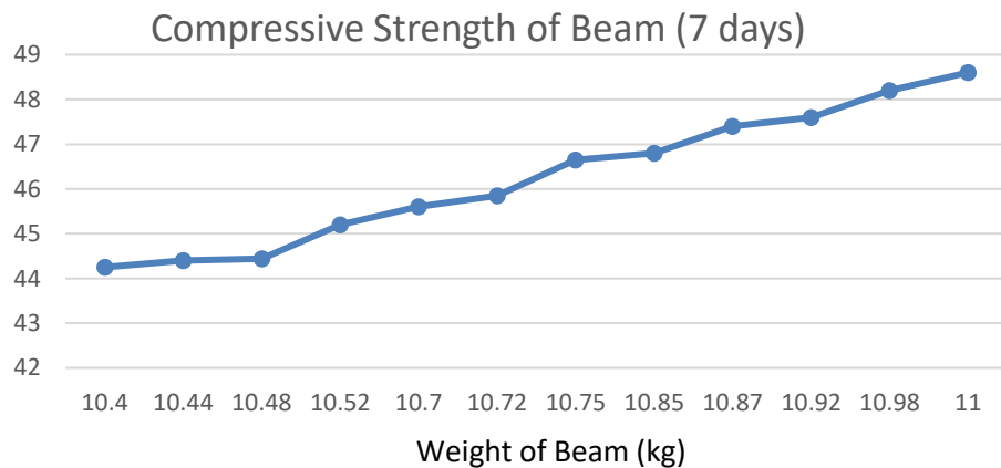
Compressive Strength of Beams for 7 days.
