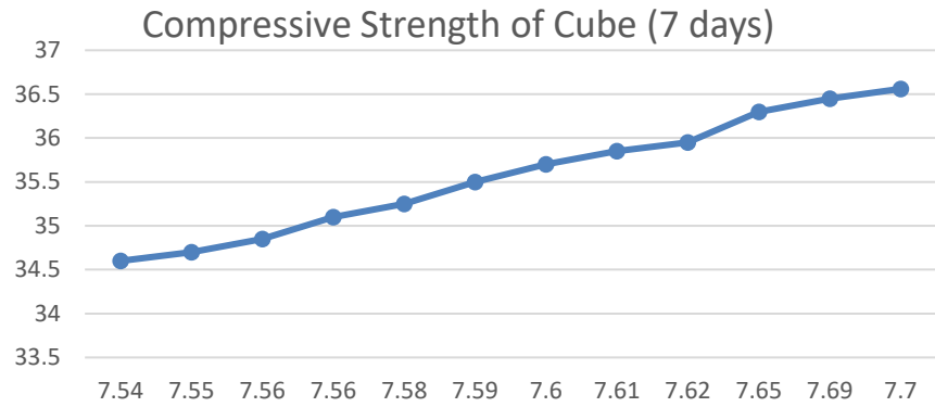
Compressive Strength of Cube for 7 days.
