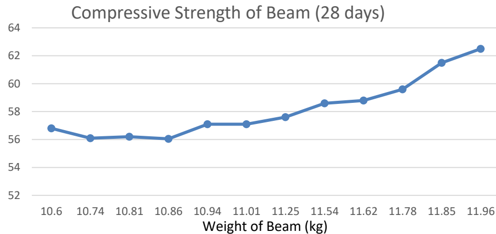
Compressive Strength of Beam for 28 days
