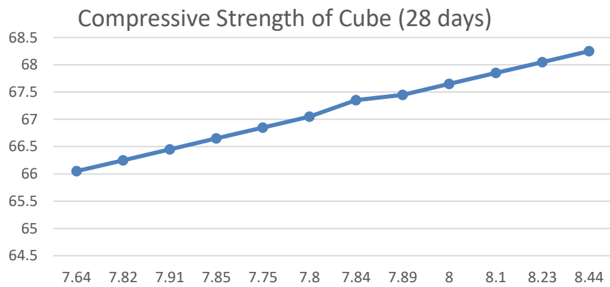
Compressive Strength of Cube for 28 days.
