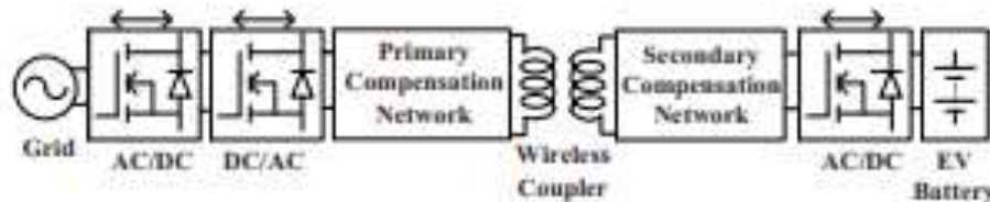
Fig -2 : Block Diagram Grid Connected BD-WPT System
