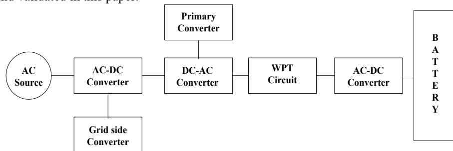
Fig -2: Block Diagram of proposed System
