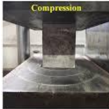
Fig. compression Testing of Cubes
