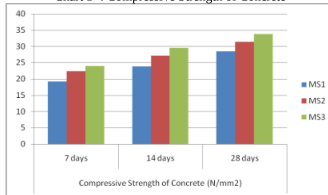
Chart 2 -: Compressive Strength of Concrete
