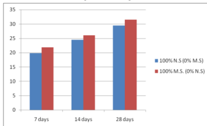
Chart 3 -: Comparison of Compressive Strength of Concrete
