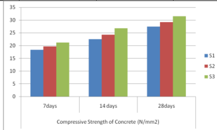
Chart 1 -: Compressive Strength of Concrete
