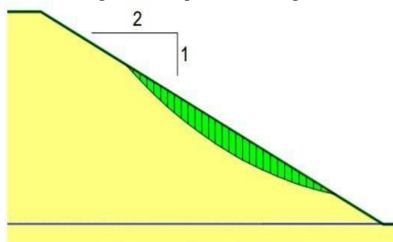
Fig -2 SLOPE/W Analysis Result with \phi value increase by 27.5%. As per literature Survey. After adding fly ash 30
