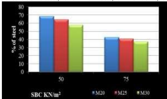
Fig. 5: Comparison of Pile & Raft foundation for 5th storey
