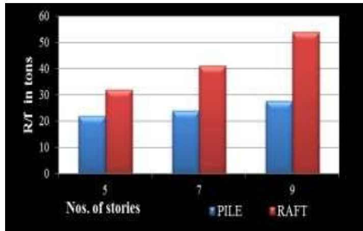
Fig. 3 Comparison of Pile & Raft foundation (M20)
