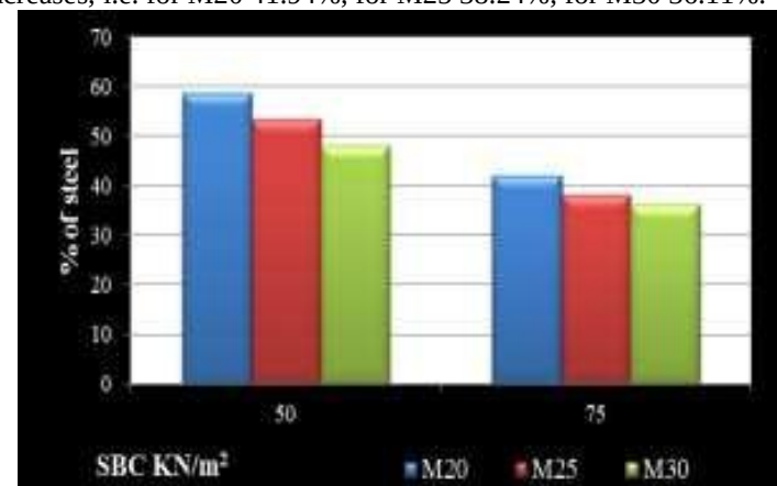
Fig. 6: Comparison of Pile & Raft foundation for 7th storey
