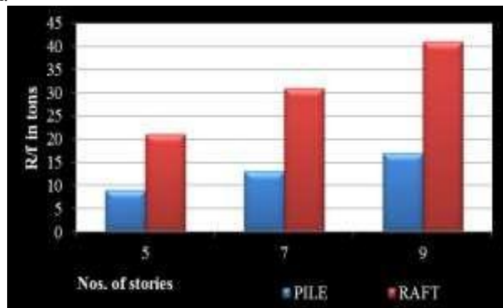
Fig. 4: Comparison of Pile & Raft foundation (M20)
