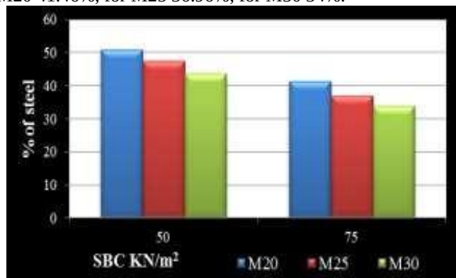
Fig. 7: Comparison of Pile & Raft foundation for 9th storey
