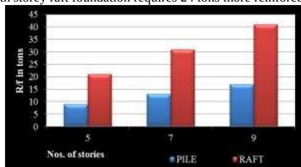
Fig. 4: Comparison of Pile & Raft foundation (M20)
