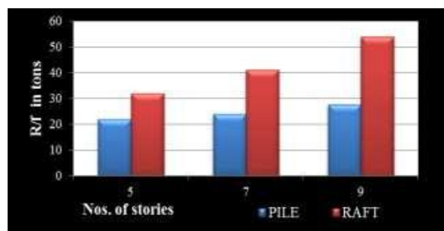
Fig. 3 Comparison of Pile & Raft foundation (M20)
