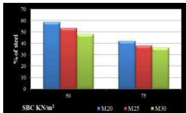
Fig. 6: Comparison of Pile & Raft foundation for 7th storey
