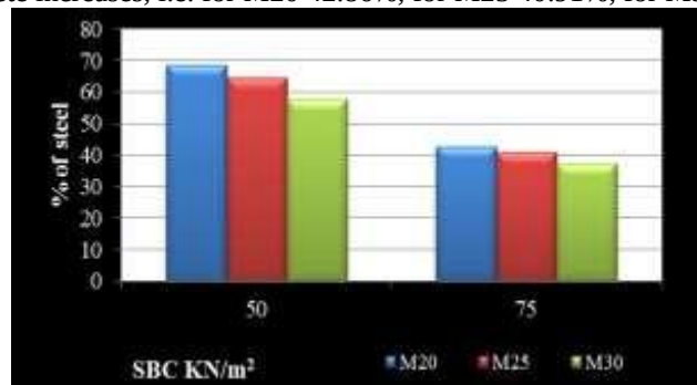
Fig. 5: Comparison of Pile & Raft foundation for 5th storey
