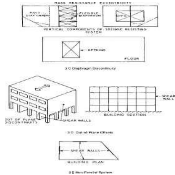
Fig. 4.5.1 Plan Irregularities
