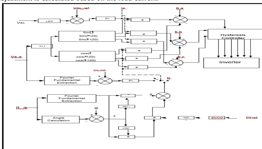
Fig.2 H-controller
