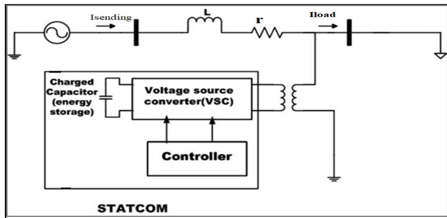
Fig. 1 STATCOM with system
