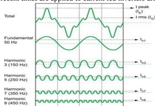
Figure: 2 Odd Harmonics
