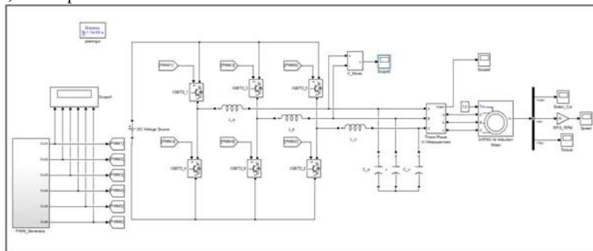
Figure 5: Simulink model with Passive Filters.
