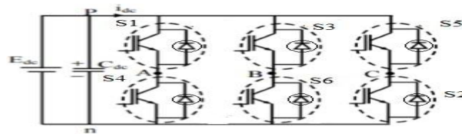
Figure 1: Inverter Circuit Diagram
