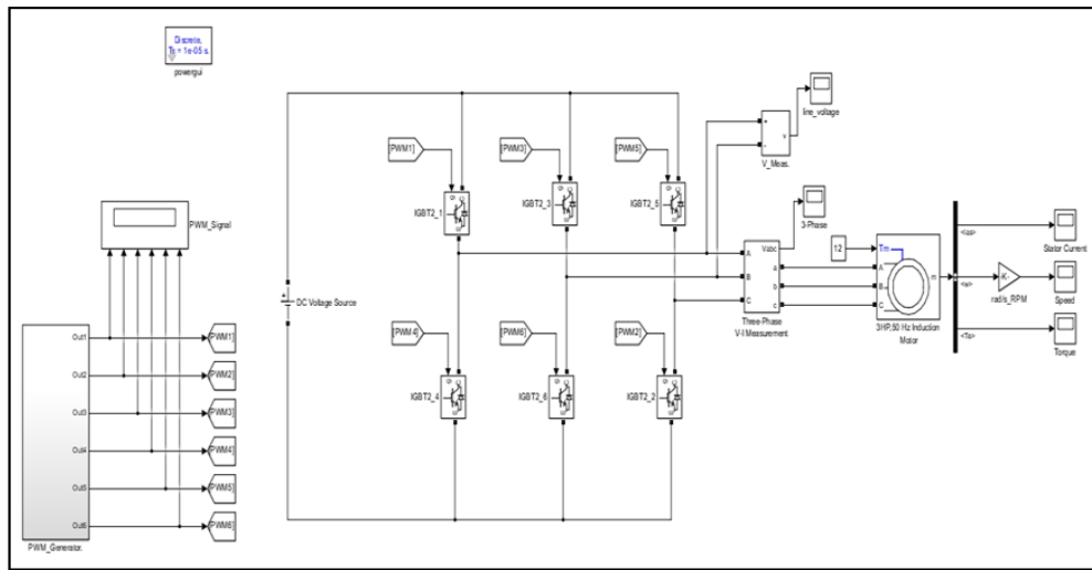
Figure 4: Simulink Model
