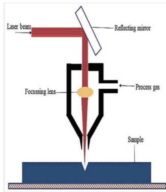
Figure-1: Schematic layout of the process
