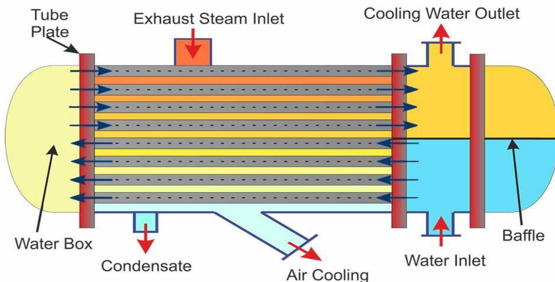
Fig -1: Steam Condenser
