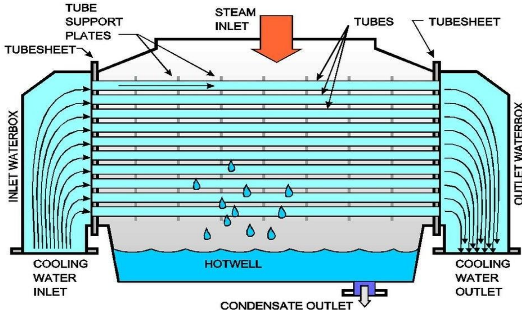
Fig -2: Representation of steam condensation
