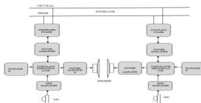
Fig 1: Block diagram of voice communication over power-line.
