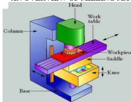
Fig.1 Milling Machine
