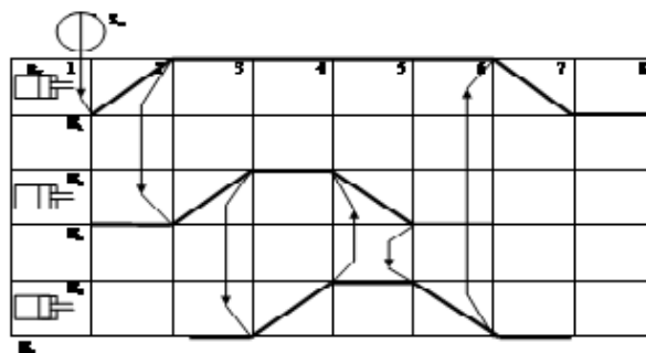
Fig. 2 Functional Diagram
