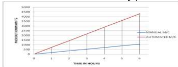
Fig. 3 Graph Showing Productivity Of Two Machines (Milling) AUTOMATED M/C/MANUAL OPERATED M/C
