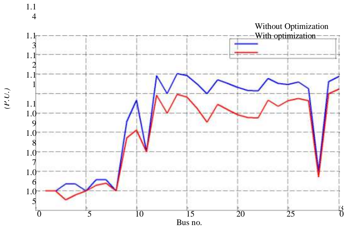
Fig: 4 Performance of Graph with and Without Optimization
